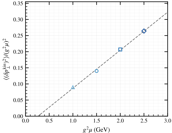
(b) Accumulated momentum in the Glasma phase
